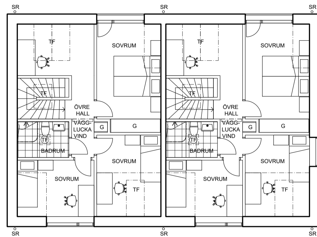
PLAN 2
