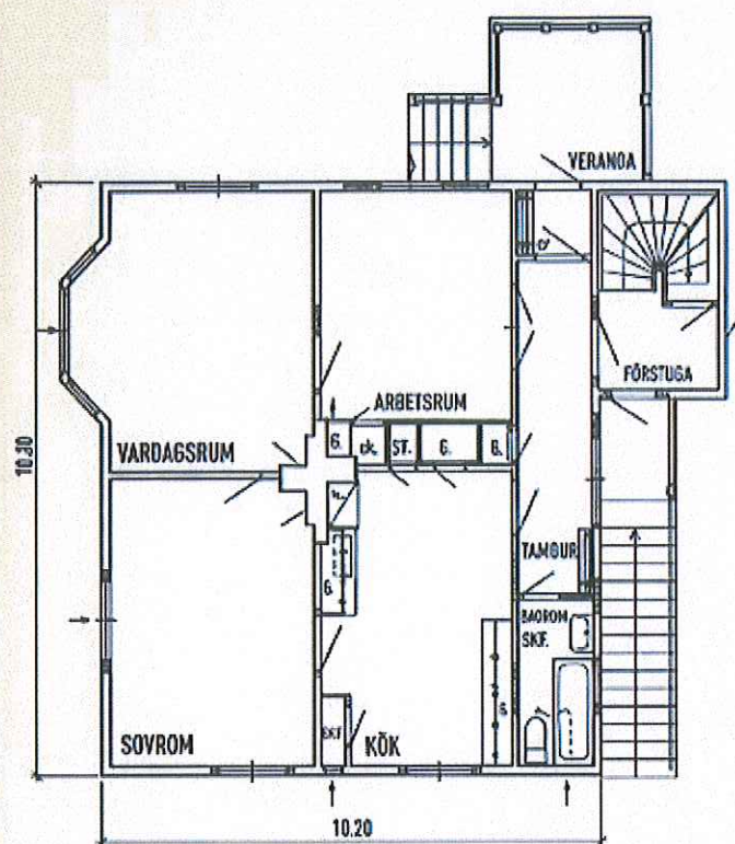
BOTTENPLAN
